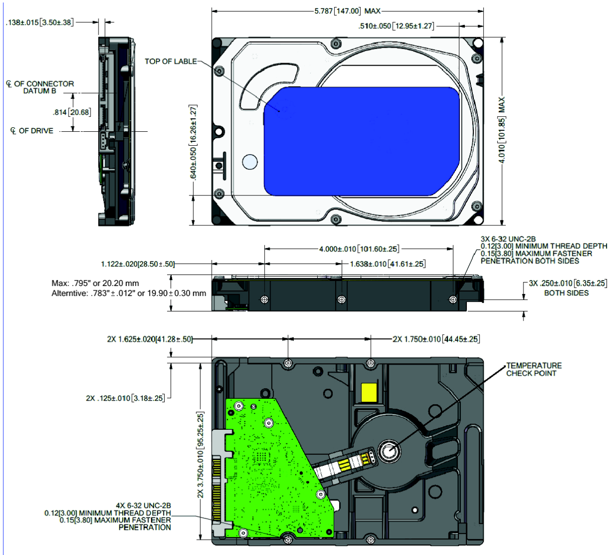
Figure 2 Mounting dimensions
