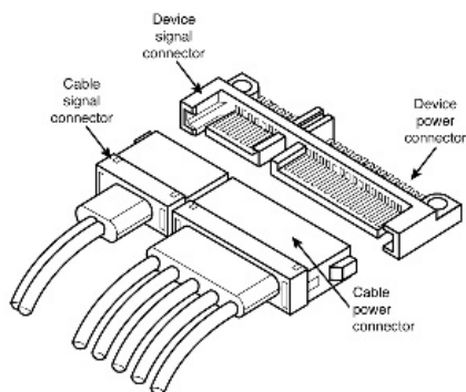
Figure 1 Attaching SATA cabling
