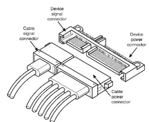
Figure 2 Attaching SATA cabling
