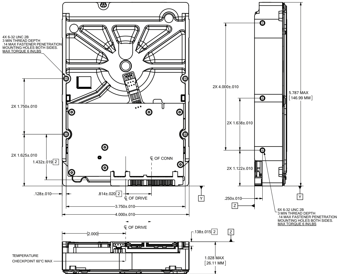
Figure 3 Mounting dimensions
