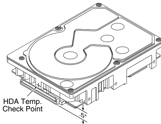
Figure 12. Location of HDA Temperature Check Point
