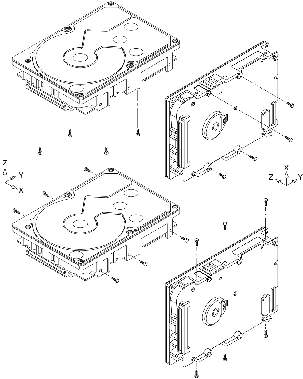
Figure 13. Recommended mounting
