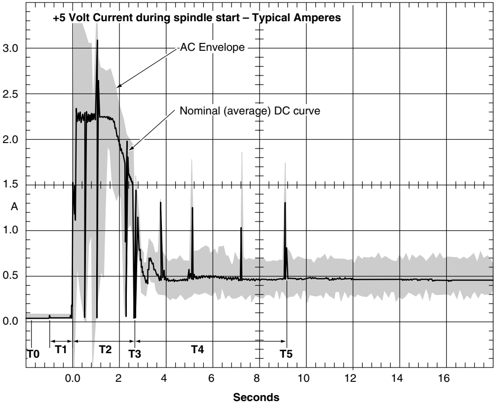
Figure 4. Typical ST318405 drive +12 V current profile
