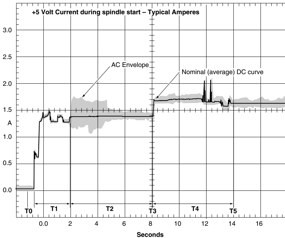
Figure 6. Typical ST336705 drive +5 V current profile
