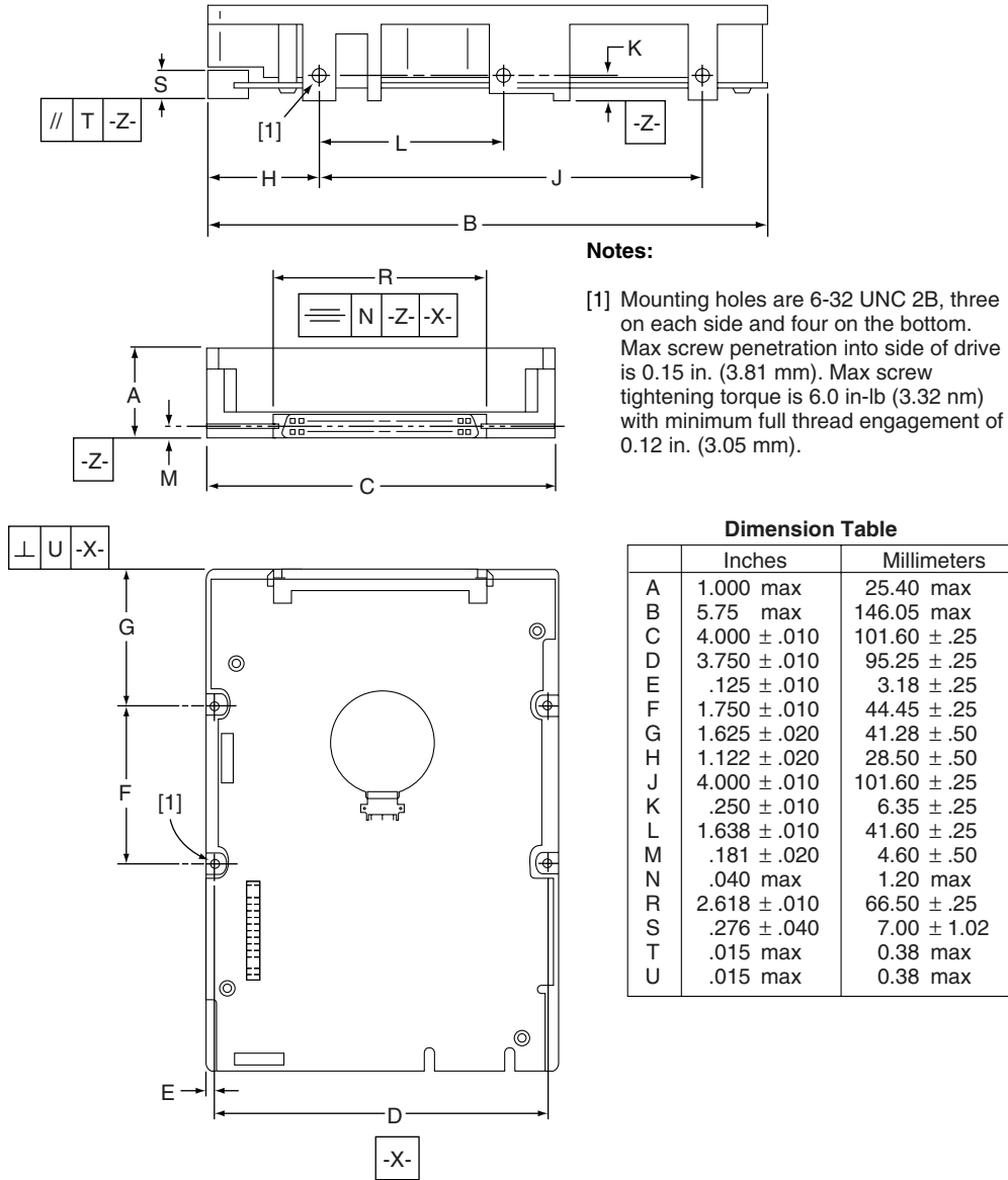
Figure 15. LC mounting configuration dimensions
