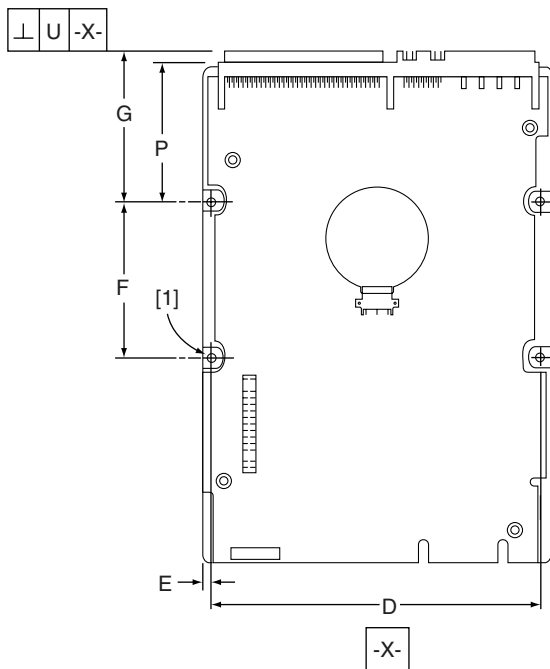
Figure 14. LW mounting configuration dimensions
