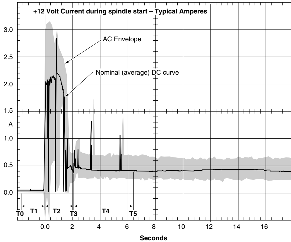
Figure 5. Typical ST39205 drive +12 V current profile
