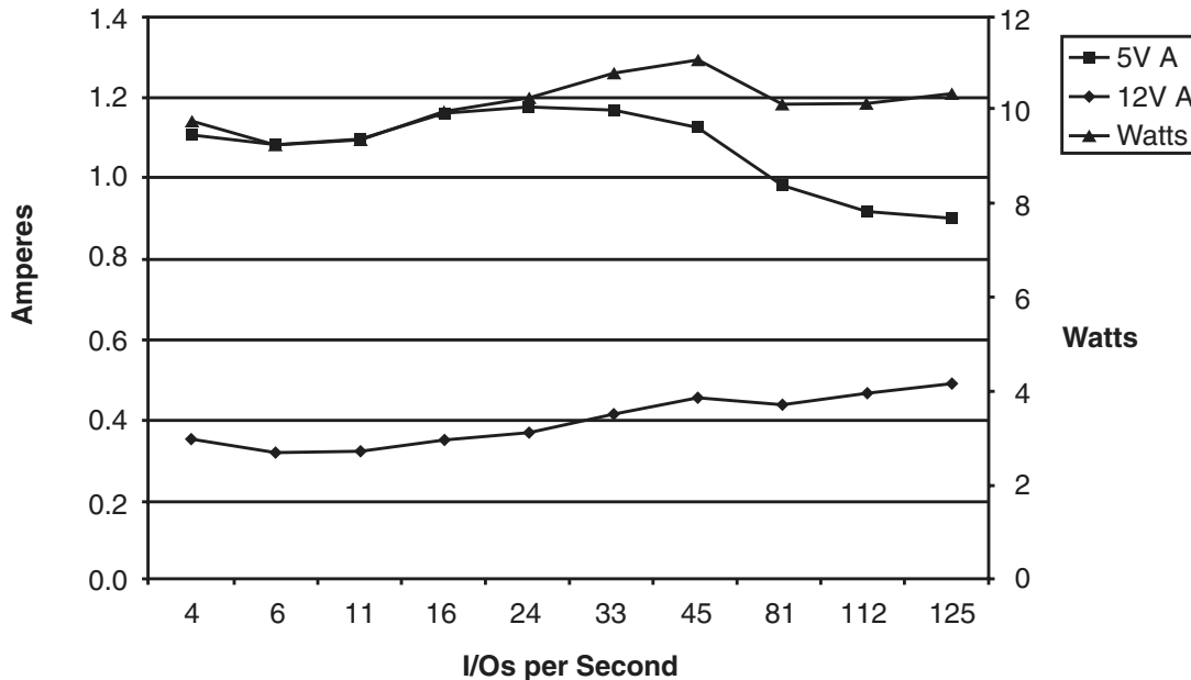
Figure 11. ST39205 DC current and power vs. input/output operations per second (LVD)
