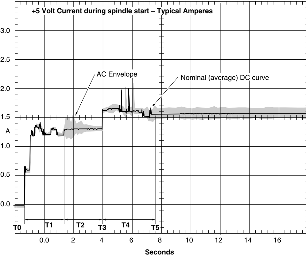
Figure 8. Typical ST39205 drive +5 V current profile
