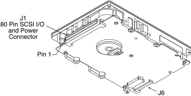
Figure 20. LC model drive physical interface (80-pin J1 SCSI I/O connector)
