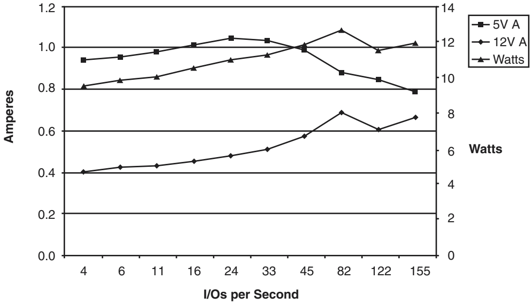
Figure 10. ST318405 DC current and power vs. input/output operations per second
