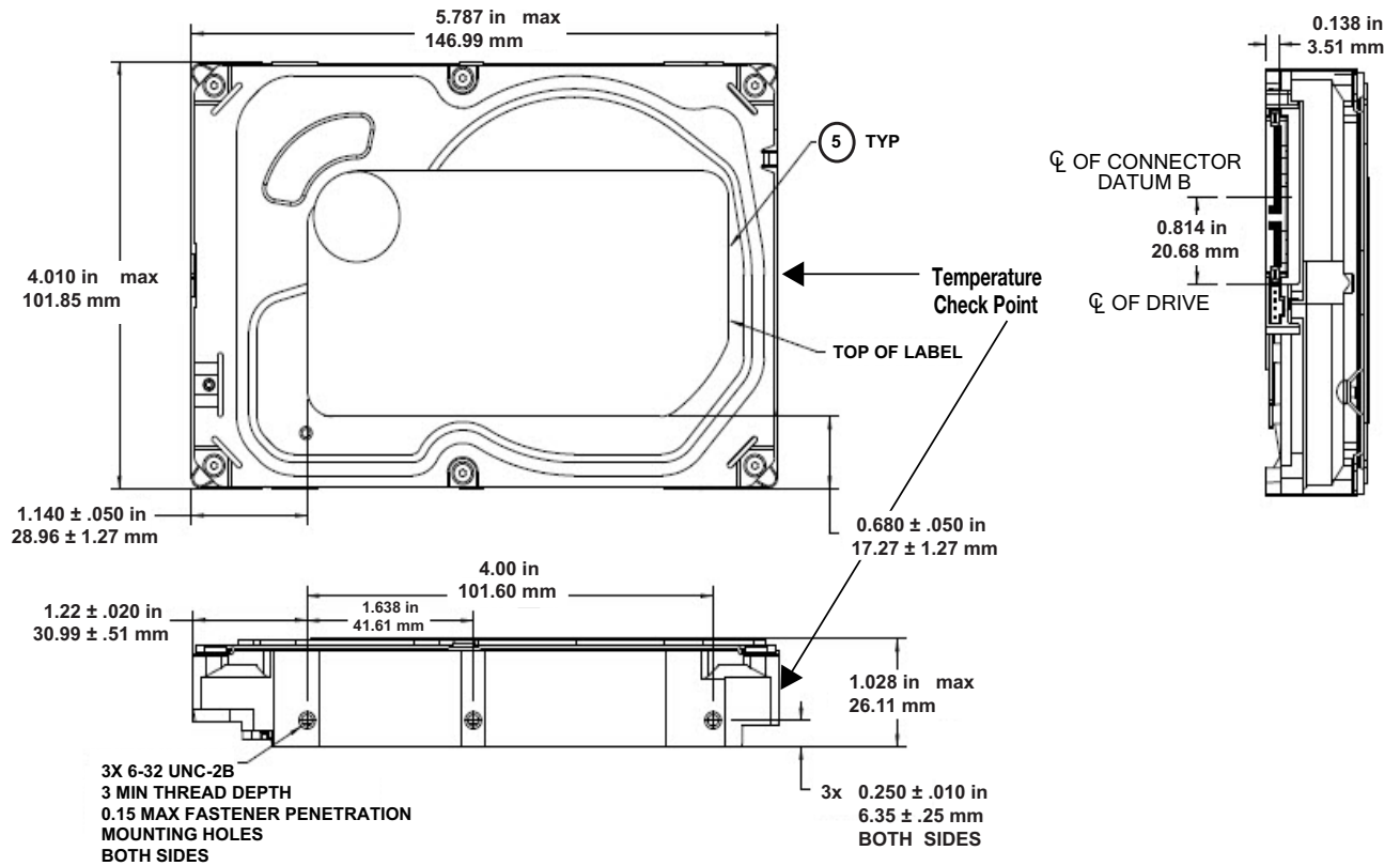
Figure 2 Mounting dimensions (2TB,3TB and 4TB)
