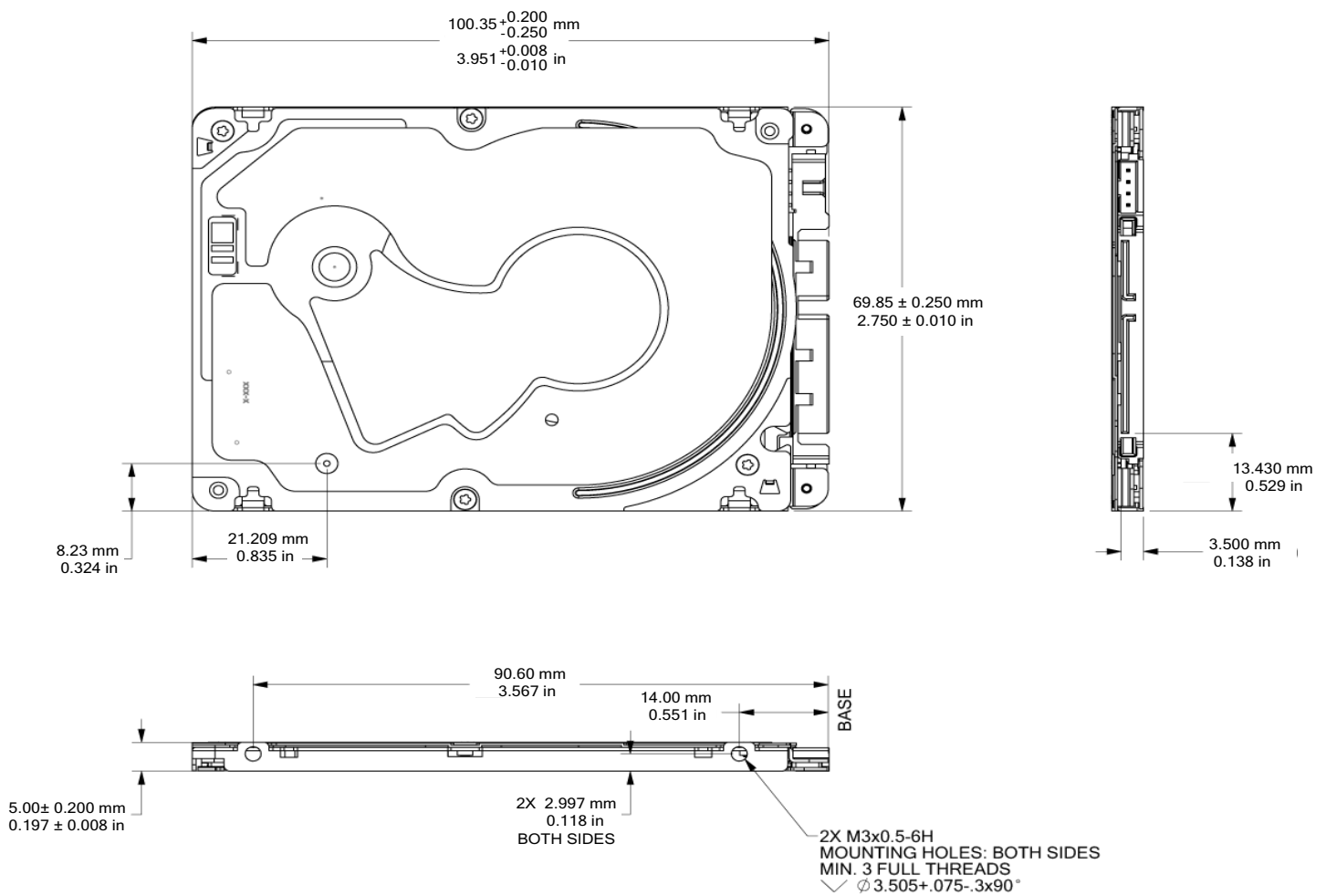
Figure 3 Mounting Dimensions (for standard models)
