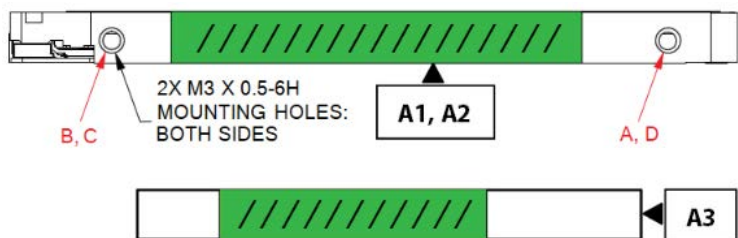
Figure 2 Drive Grounding Side Mounting for 1-disk and 2-disk models)
