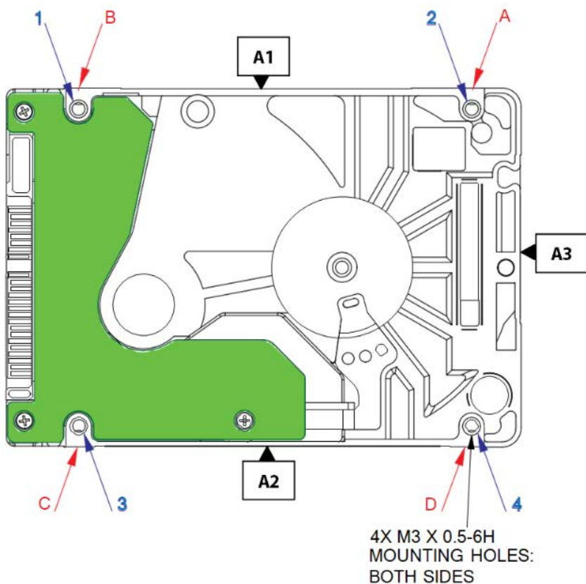
Figure 3 Drive Grounding Bottom Mounting for 1-disk and 2-disk models
