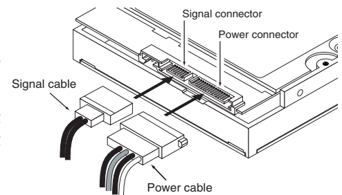
Figure 1 Attaching SATA Cabling
