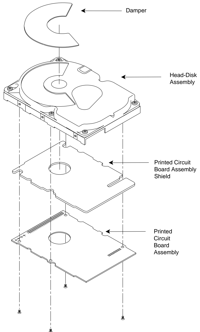
Figure 1-1 Drive Top Level Assembly
