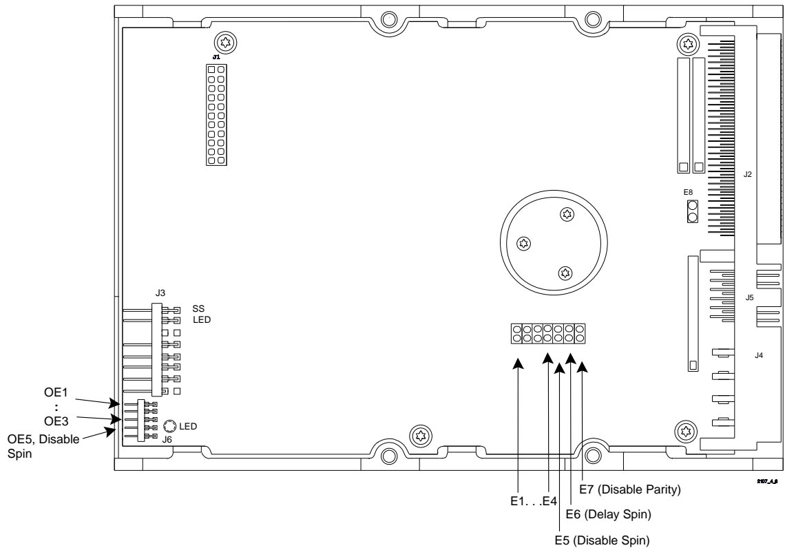
Figure 4-6 Jumper Locations
