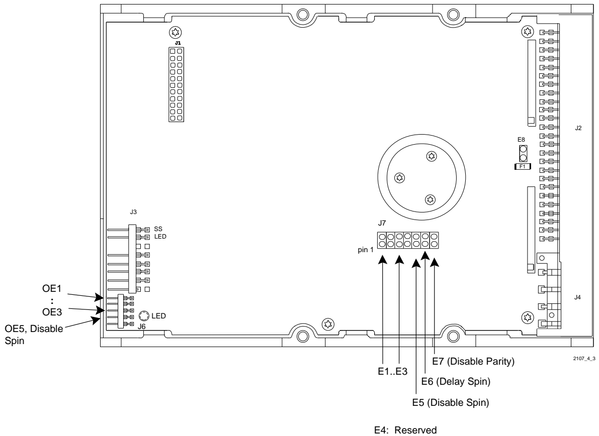
Figure 4-3 Jumper Locations
