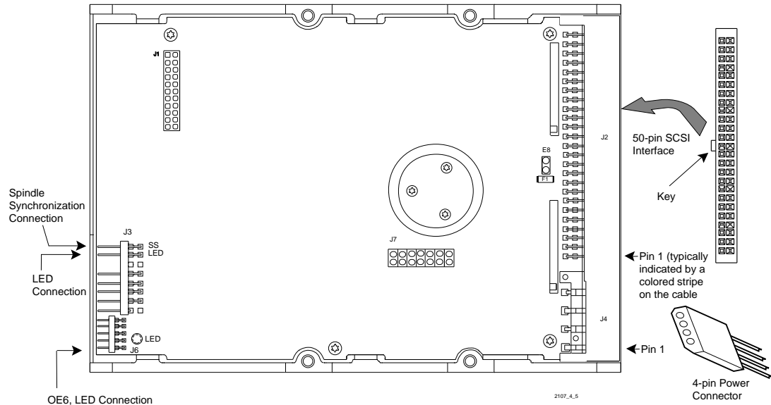
Figure 4-5 Connecting the cabling
