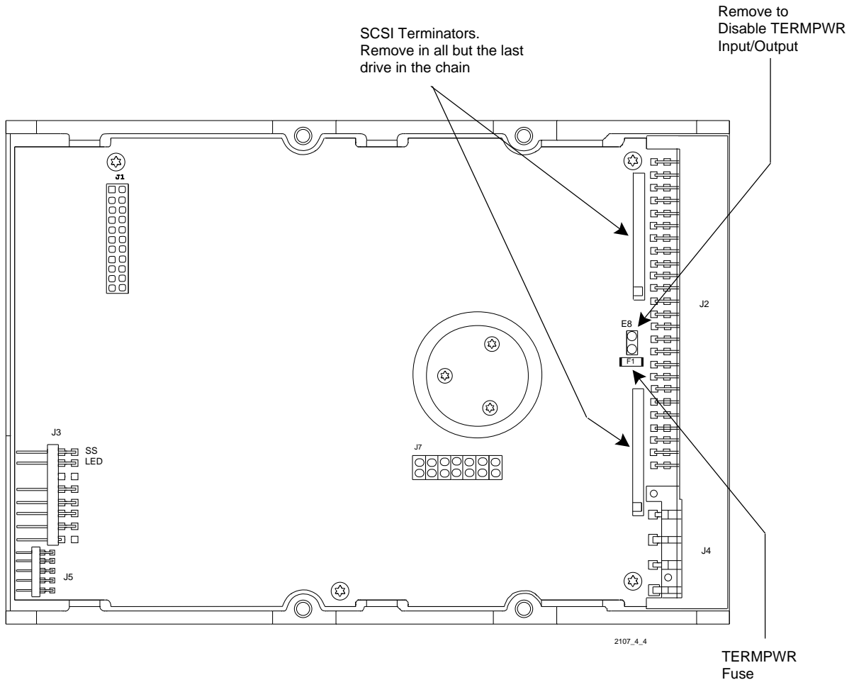
Figure 4-4 Terminator Resistor Locations
