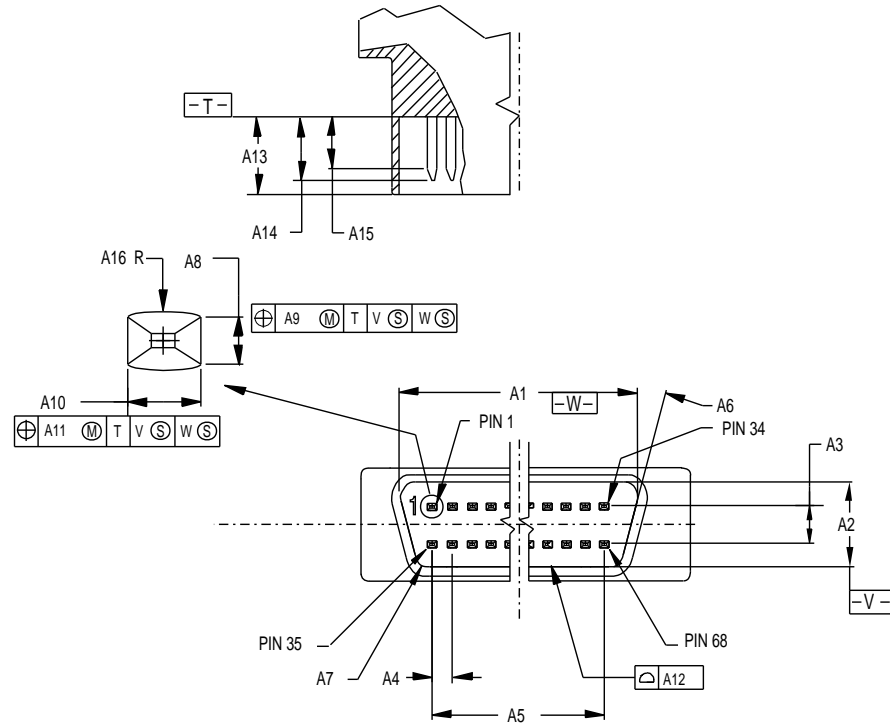
Figure 5-4 P-Cable Connector
