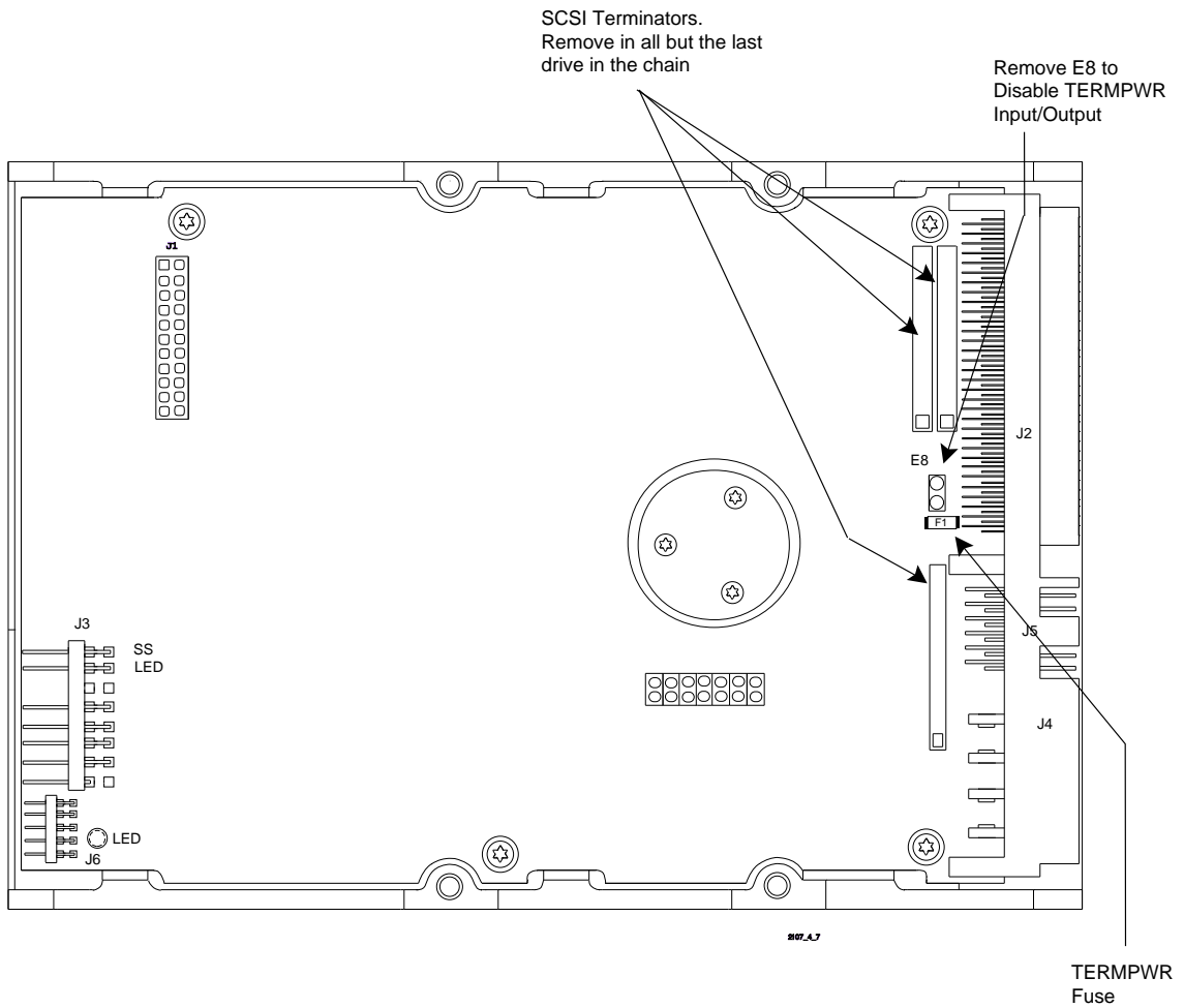
Figure 4-7 Terminator Resistor Locations
