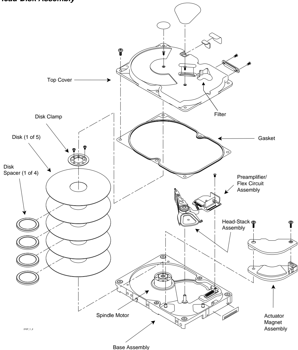
Figure 1-2 Head-Disk Assembly
