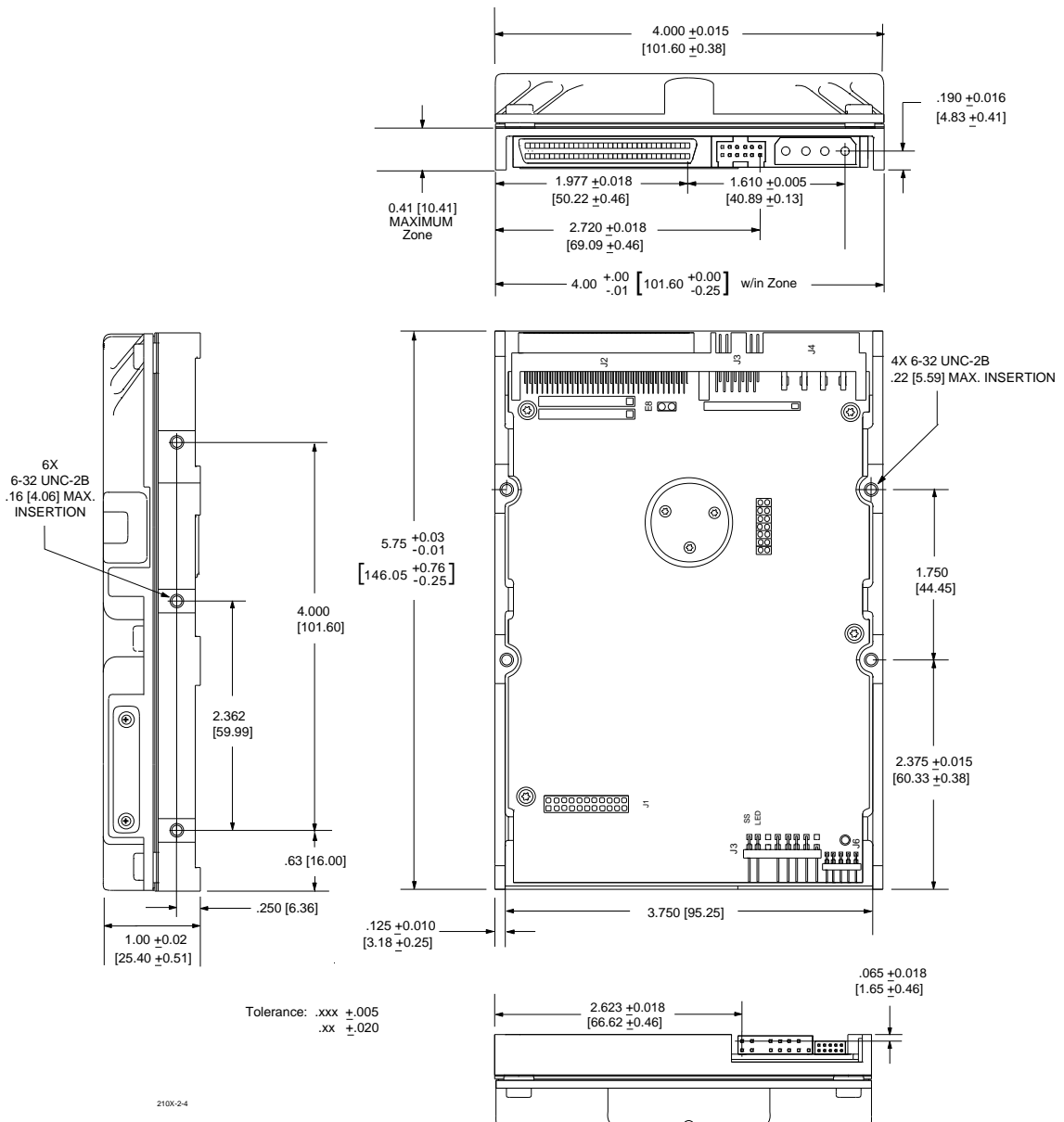
Figure 2-4 The Drive's Physical Dimensions
